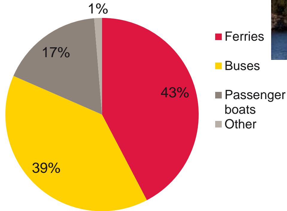
CO2-emissions in 2014, tonn
